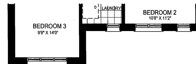
SECOND FLOOR PLAN ELEVATION 'B'
