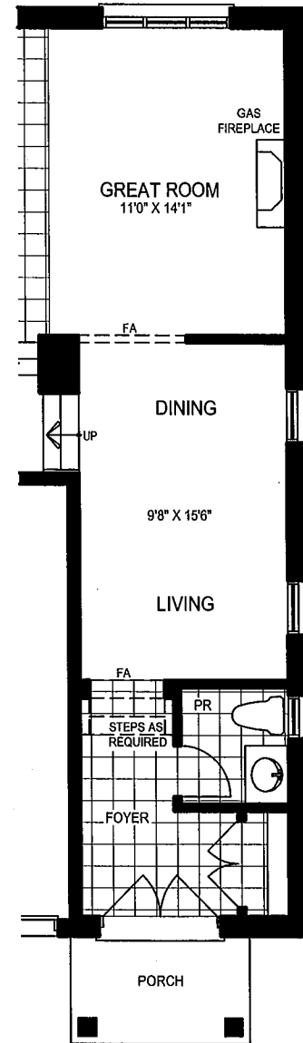
OPTIONAL GROUND FLOOR PLAN
